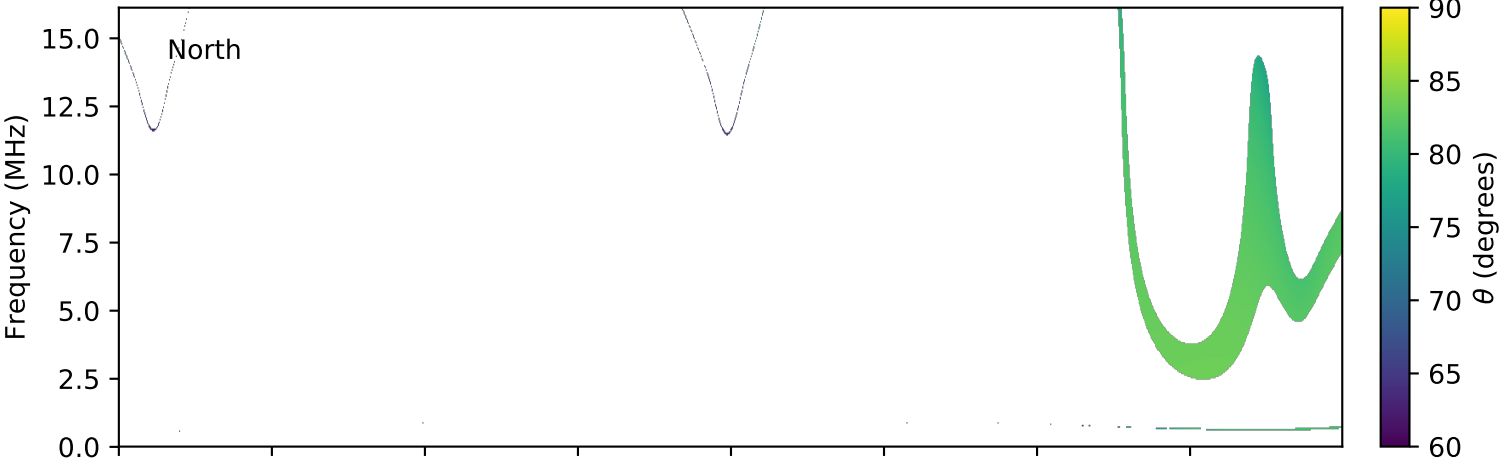
expres_cassini_jupiter_europa_isaac_lossc-wid1deg_3kev_20000526_v01.cdf
