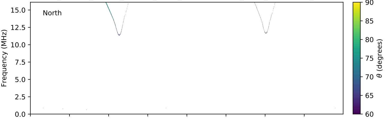
expres_cassini_jupiter_europa_isaac_lossc-wid1deg_3kev_20000522_v01.cdf
