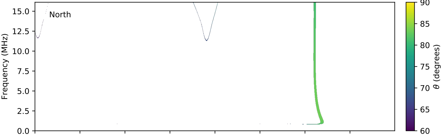
expres_cassini_jupiter_europa_isaac_lossc-wid1deg_3kev_20000519_v01.cdf
