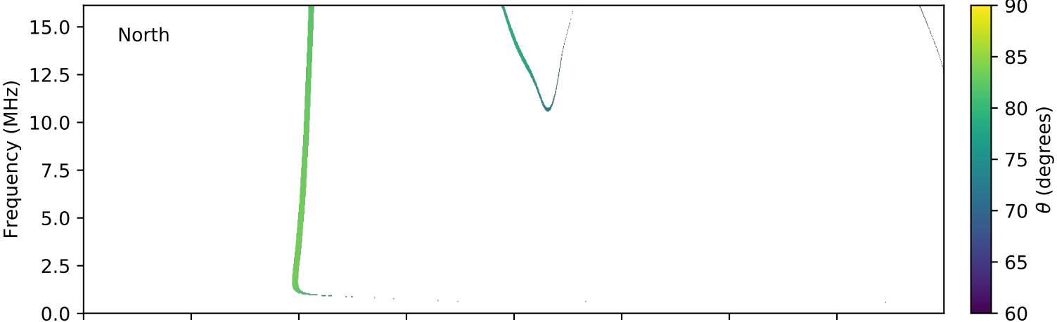
expres_cassini_jupiter_europa_isaac_lossc-wid1deg_3kev_20000518_v01.cdf
