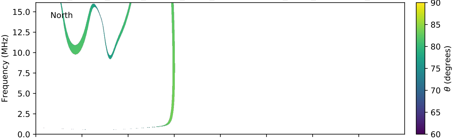
expres_cassini_jupiter_europa_isaac_lossc-wid1deg_3kev_20000516_v01.cdf
