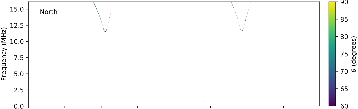
expres_cassini_jupiter_europa_isaac_lossc-wid1deg_3kev_20000515_v01.cdf
