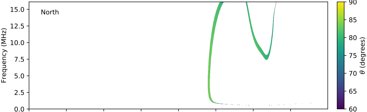
expres_cassini_jupiter_europa_isaac_lossc-wid1deg_3kev_20000514_v01.cdf
