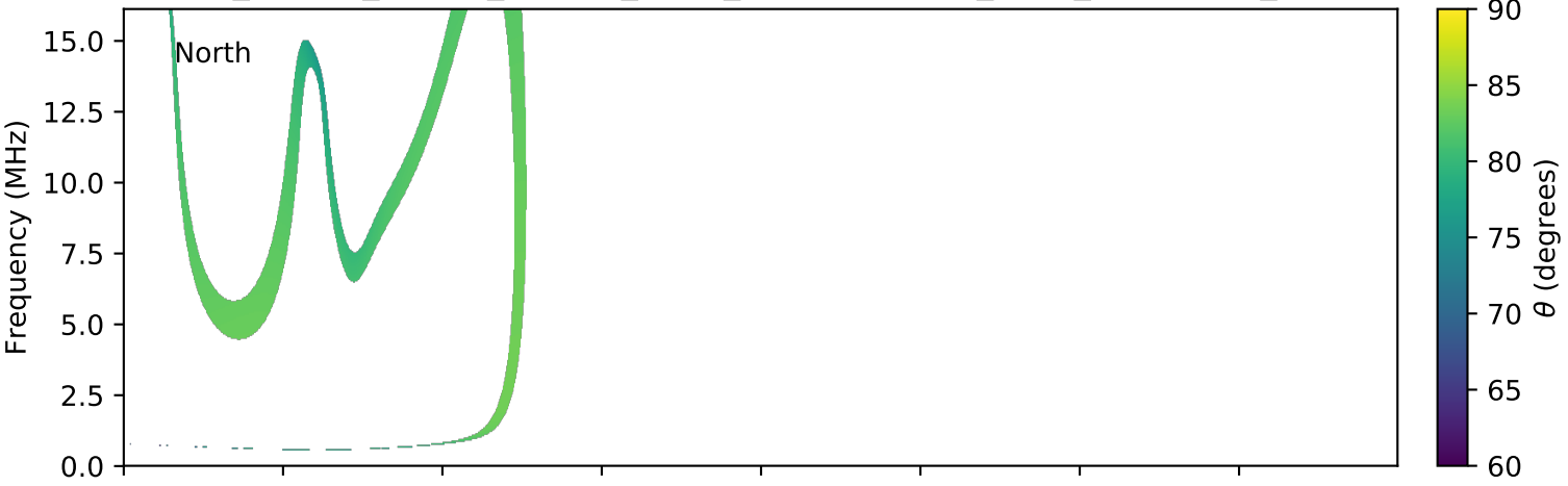
expres_cassini_jupiter_europa_isaac_lossc-wid1deg_3kev_20000509_v01.cdf
