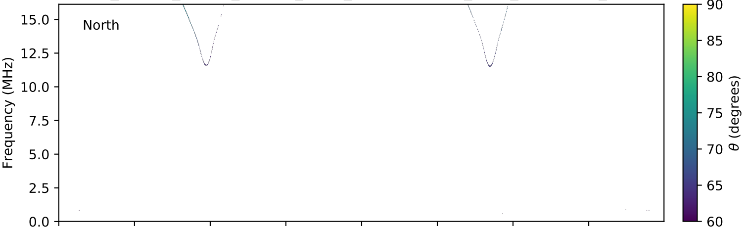
expres_cassini_jupiter_europa_isaac_lossc-wid1deg_3kev_20000508_v01.cdf
