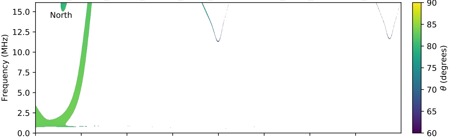
expres_cassini_jupiter_europa_isaac_lossc-wid1deg_3kev_20000504_v01.cdf
