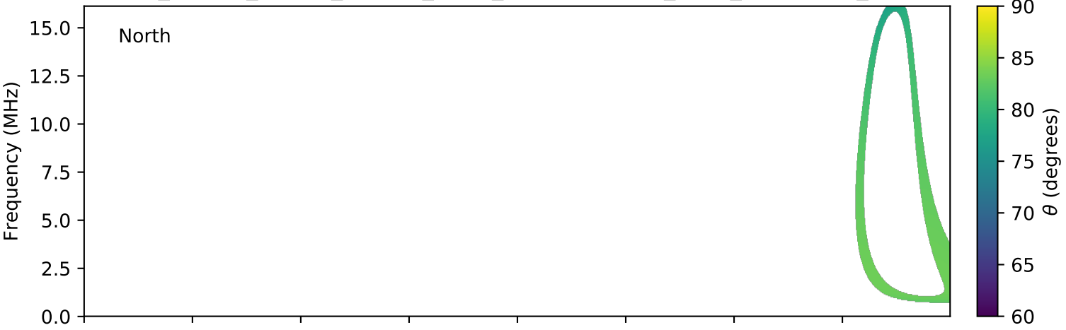
expres_cassini_jupiter_europa_isaac_lossc-wid1deg_3kev_20000503_v01.cdf
