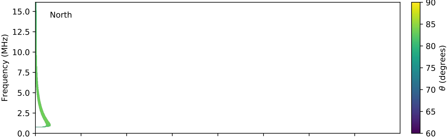
expres_cassini_jupiter_europa_isaac_lossc-wid1deg_3kev_20000502_v01.cdf
