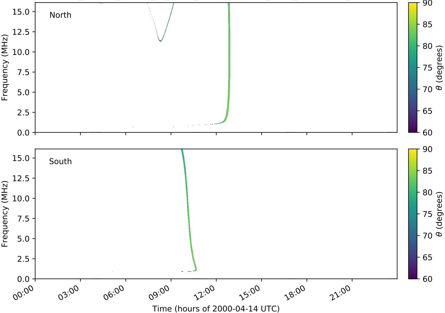
expres_cassini_jupiter_io_isaac_lossc-wid1deg_3kev_20000414_v01.cdf
