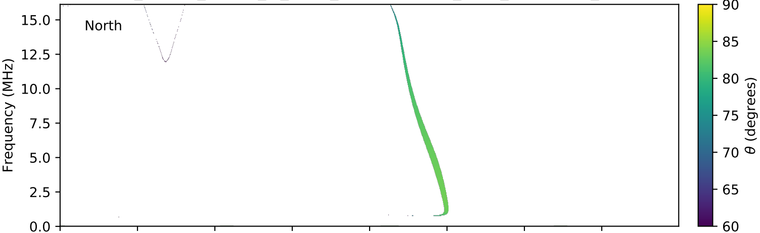
expres_cassini_jupiter_io_isaac_lossc-wid1deg_3kev_20000405_v01.cdf
