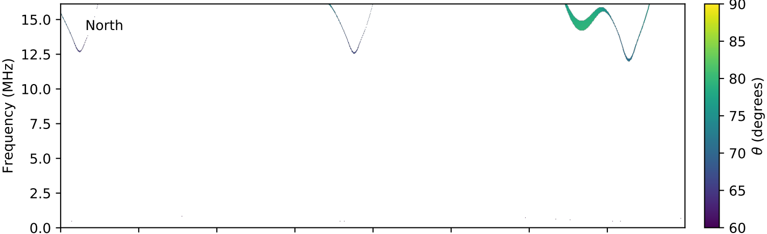
expres_cassini_jupiter_ganymede_isaac_lossc-wid1deg_3kev_20000425_v01.cdf
