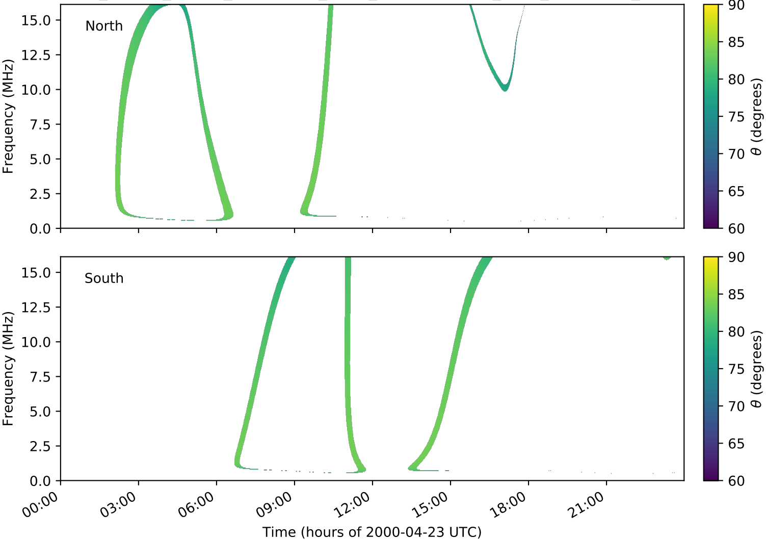
expres_cassini_jupiter_ganymede_isaac_lossc-wid1deg_3kev_20000423_v01.cdf
