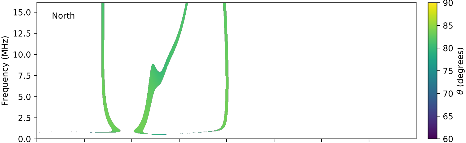
expres_cassini_jupiter_ganymede_isaac_lossc-wid1deg_3kev_20000419_v01.cdf
