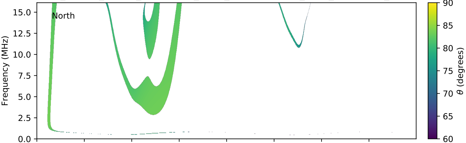
expres_cassini_jupiter_ganymede_isaac_lossc-wid1deg_3kev_20000416_v01.cdf
