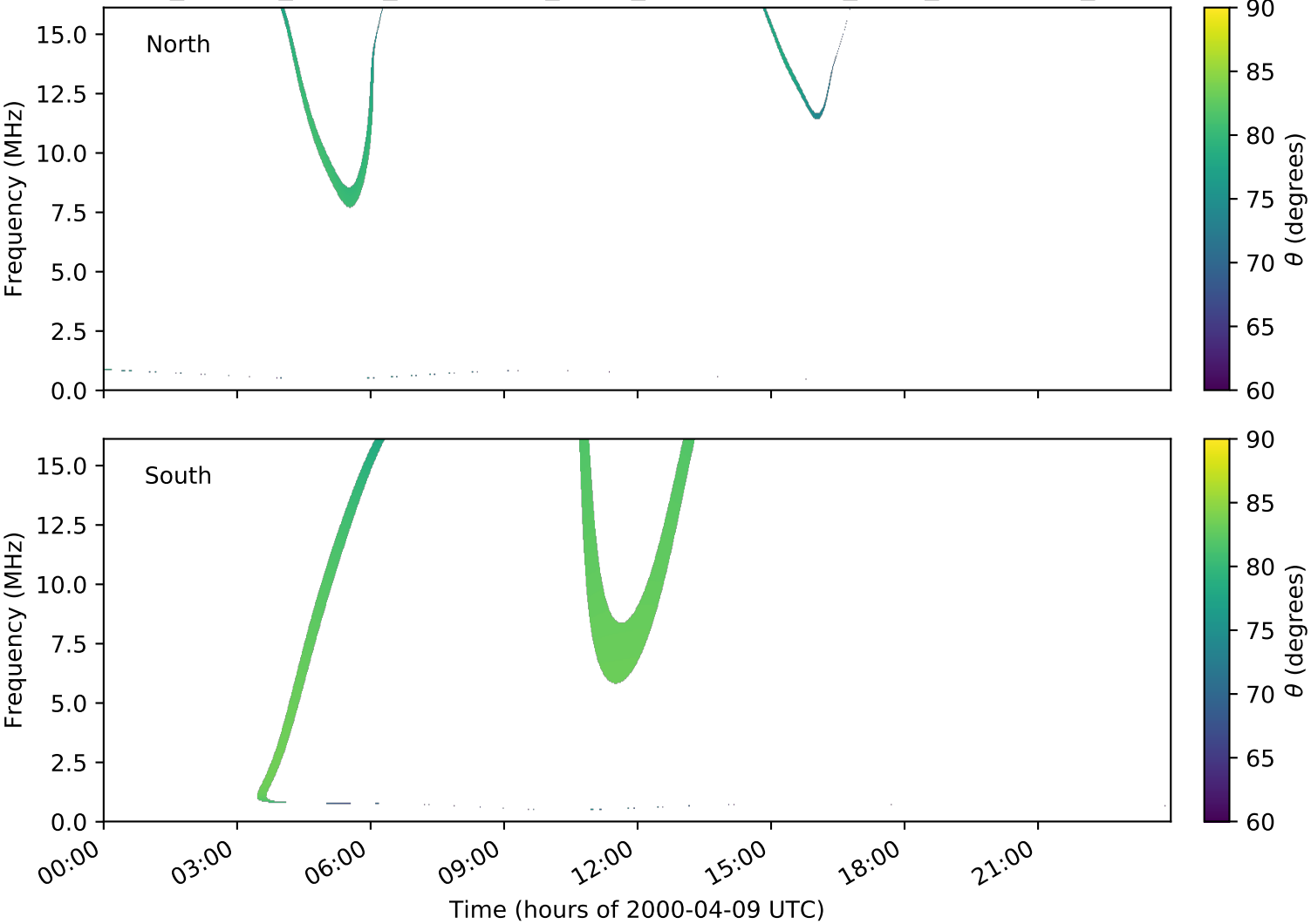
expres_cassini_jupiter_ganymede_isaac_lossc-wid1deg_3kev_20000409_v01.cdf
