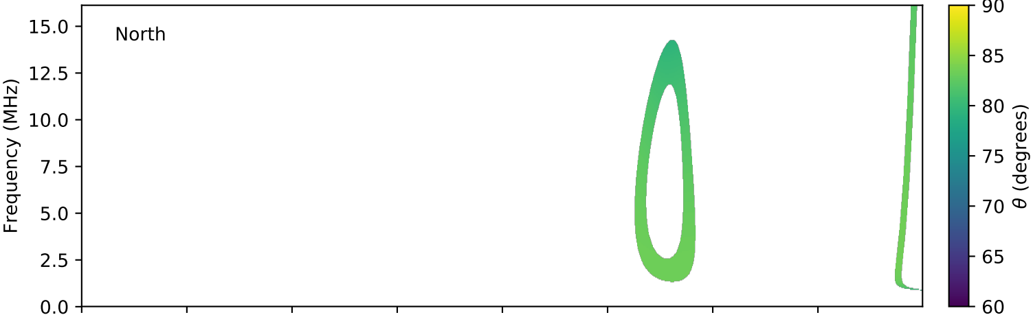
expres_cassini_jupiter_ganymede_isaac_lossc-wid1deg_3kev_20000408_v01.cdf
