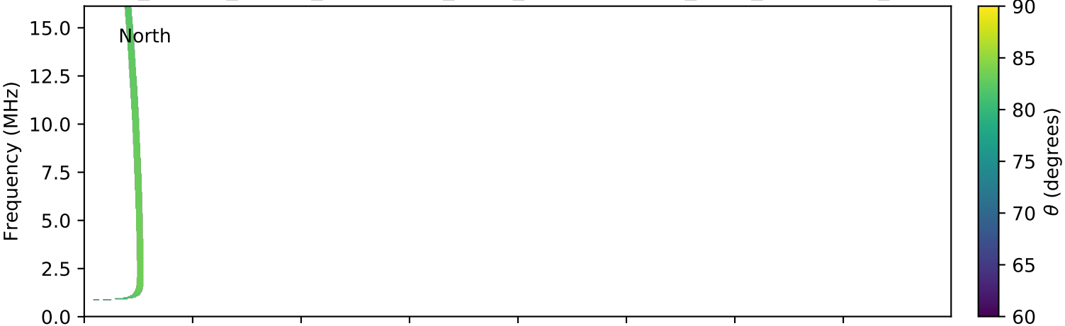
expres_cassini_jupiter_ganymede_isaac_lossc-wid1deg_3kev_20000405_v01.cdf
