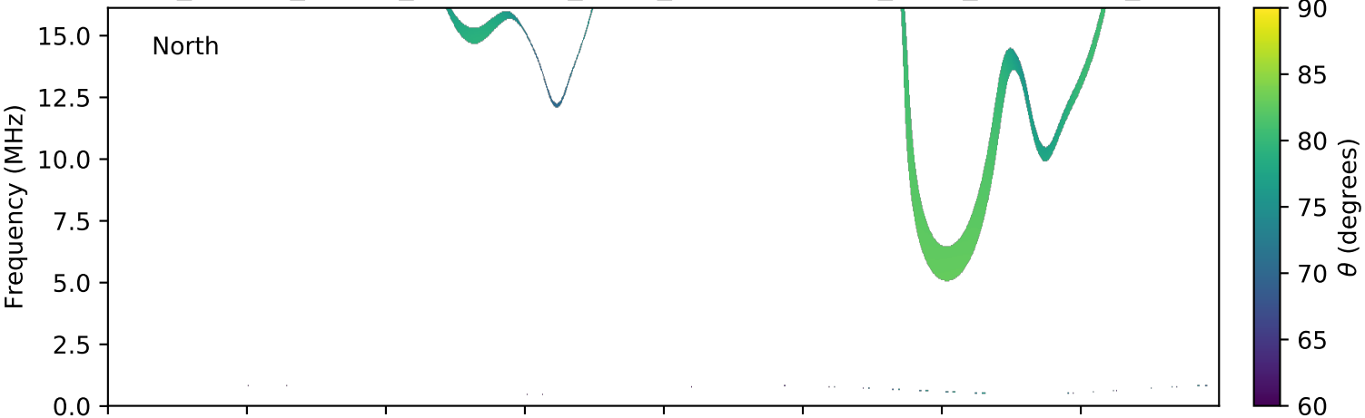
expres_cassini_jupiter_ganymede_isaac_lossc-wid1deg_3kev_20000404_v01.cdf
