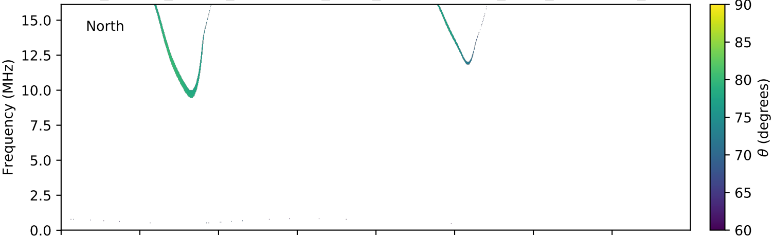
expres_cassini_jupiter_ganymede_isaac_lossc-wid1deg_3kev_20000402_v01.cdf
