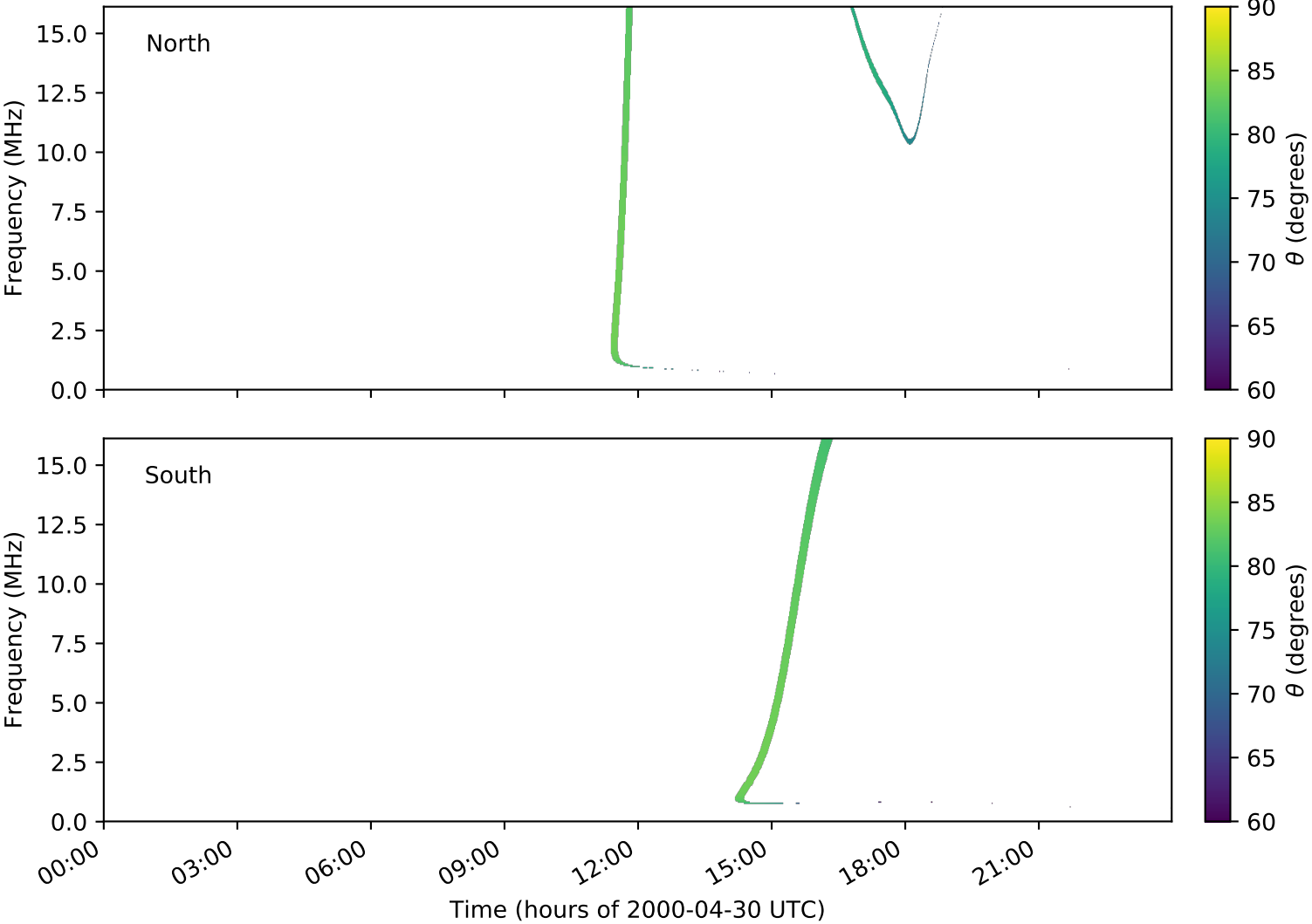
expres_cassini_jupiter_europa_isaac_lossc-wid1deg_3kev_20000430_v01.cdf
