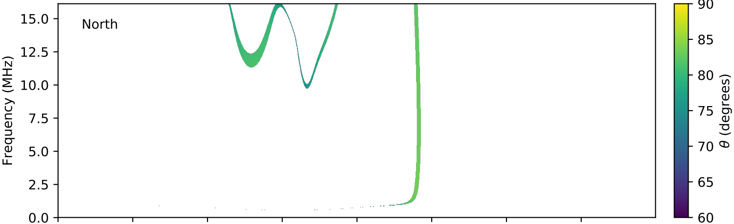
expres_cassini_jupiter_europa_isaac_lossc-wid1deg_3kev_20000428_v01.cdf
