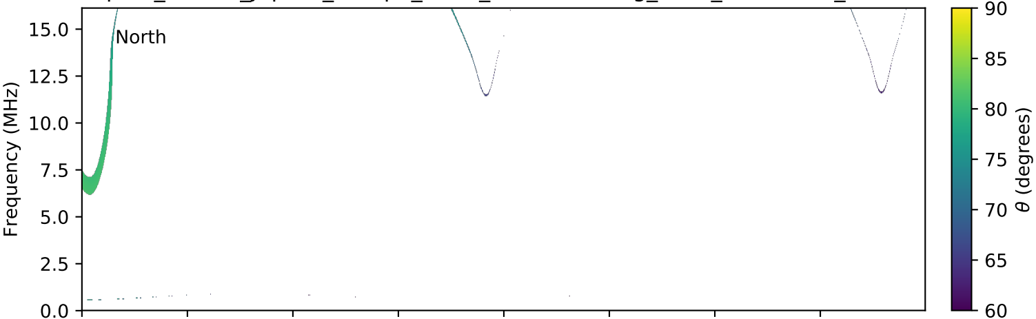
expres_cassini_jupiter_europa_isaac_lossc-wid1deg_3kev_20000427_v01.cdf
