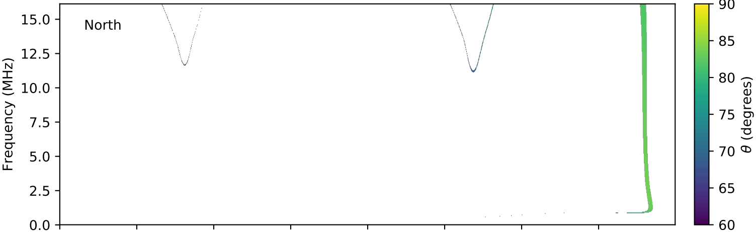
expres_cassini_jupiter_europa_isaac_lossc-wid1deg_3kev_20000424_v01.cdf
