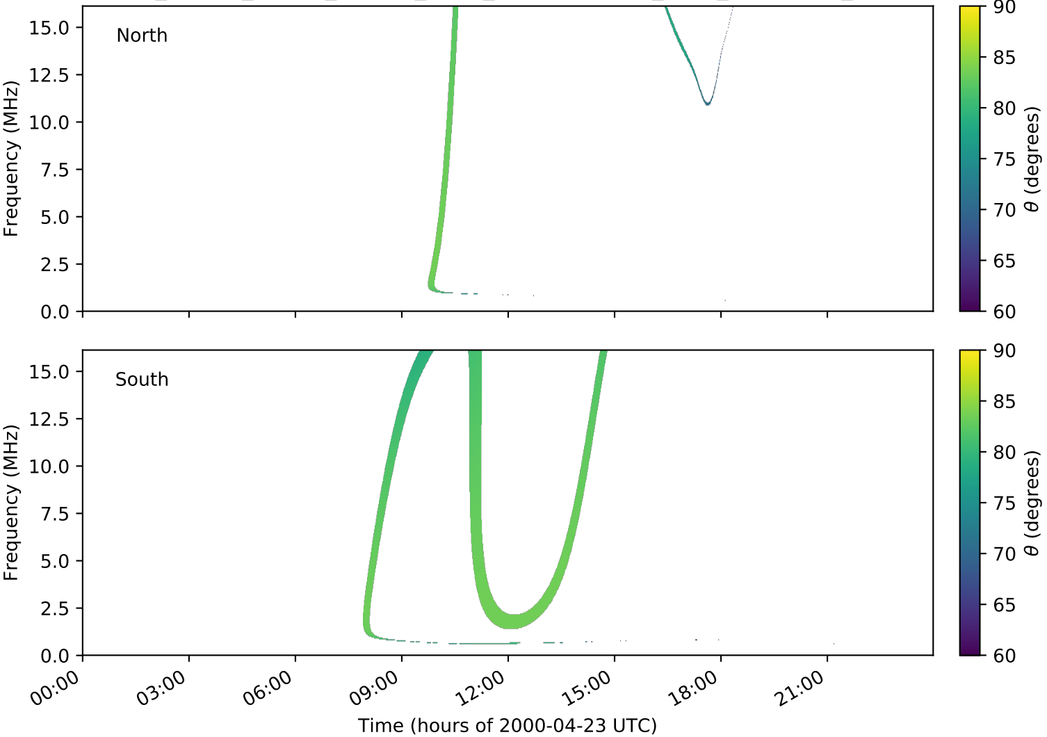
expres_cassini_jupiter_europa_isaac_lossc-wid1deg_3kev_20000423_v01.cdf
