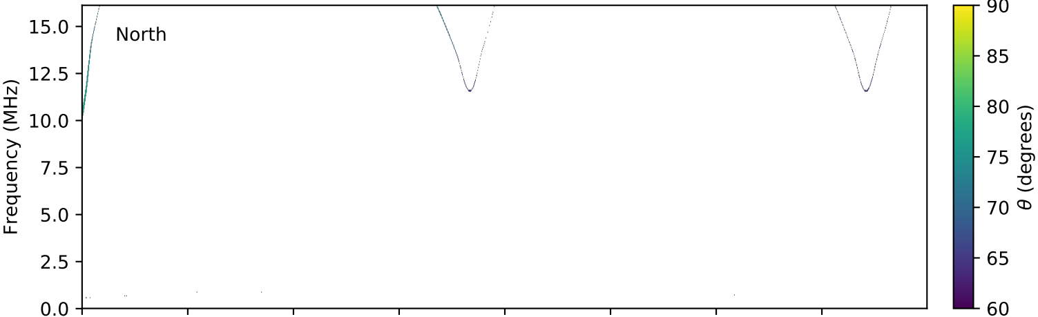
expres_cassini_jupiter_europa_isaac_lossc-wid1deg_3kev_20000420_v01.cdf
