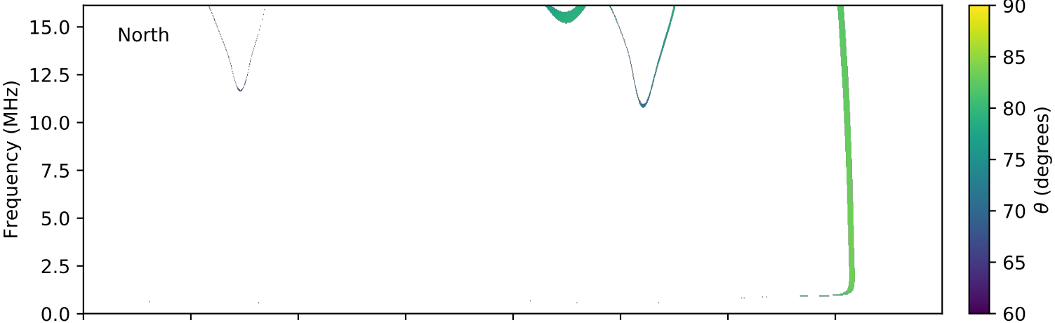
expres_cassini_jupiter_europa_isaac_lossc-wid1deg_3kev_20000417_v01.cdf
