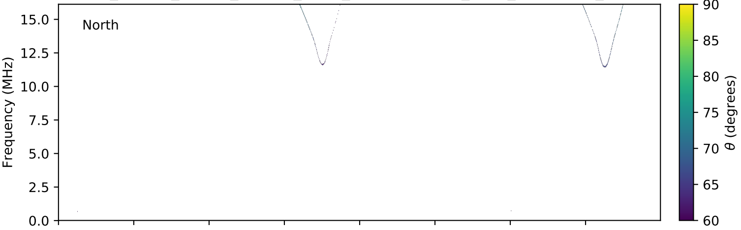
expres_cassini_jupiter_europa_isaac_lossc-wid1deg_3kev_20000413_v01.cdf
