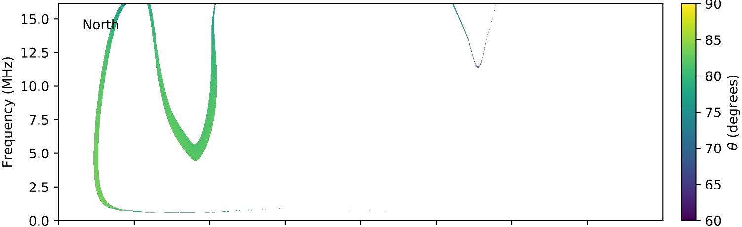
expres_cassini_jupiter_europa_isaac_lossc-wid1deg_3kev_20000409_v01.cdf
