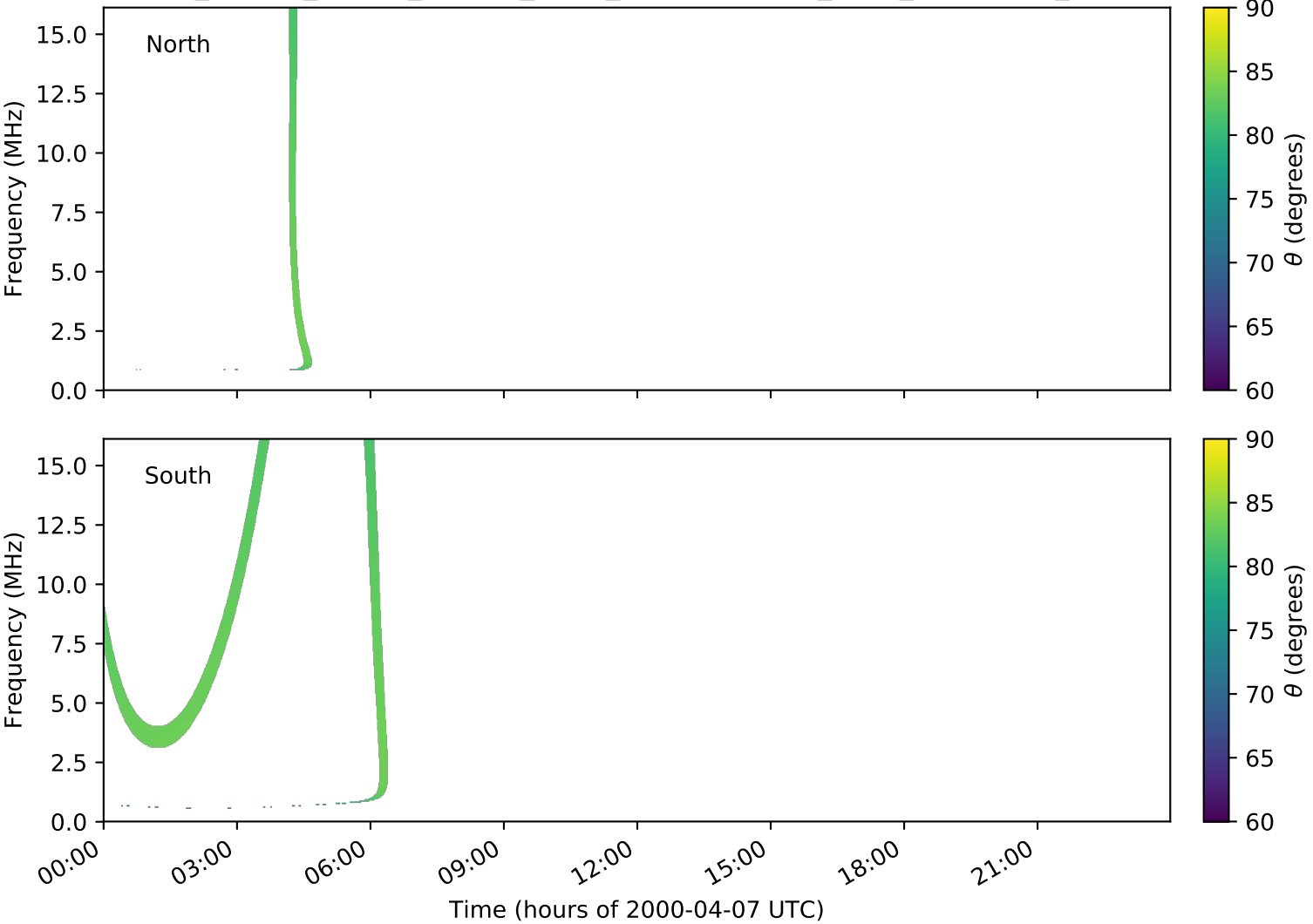
expres_cassini_jupiter_europa_isaac_lossc-wid1deg_3kev_20000407_v01.cdf
