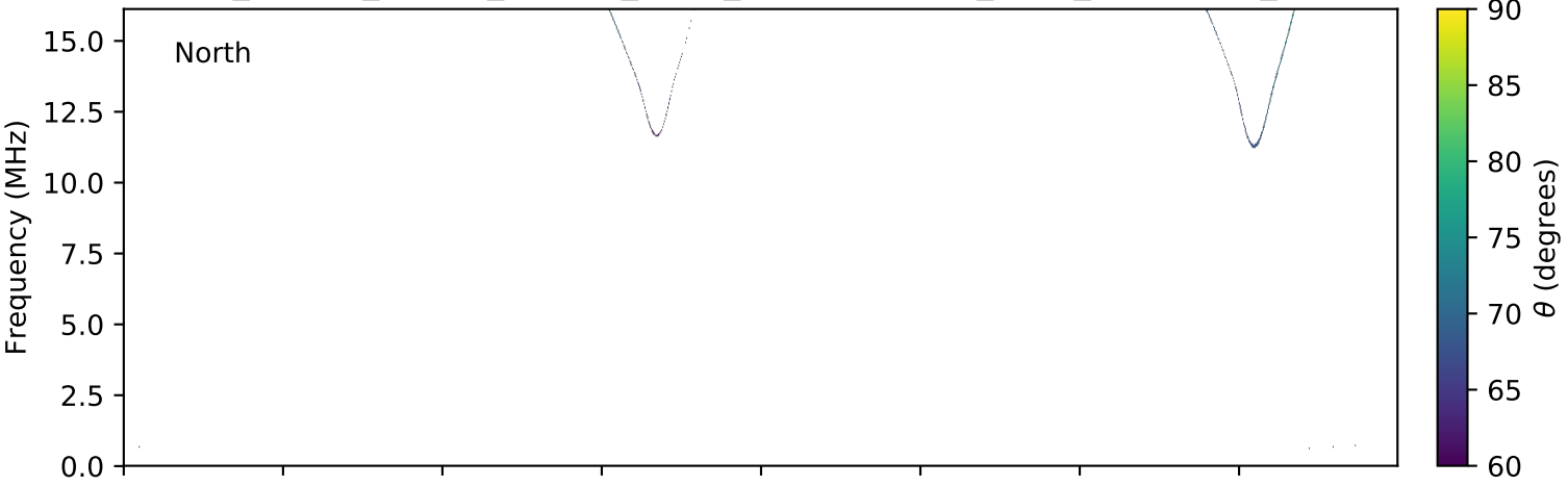
expres_cassini_jupiter_europa_isaac_lossc-wid1deg_3kev_20000406_v01.cdf
