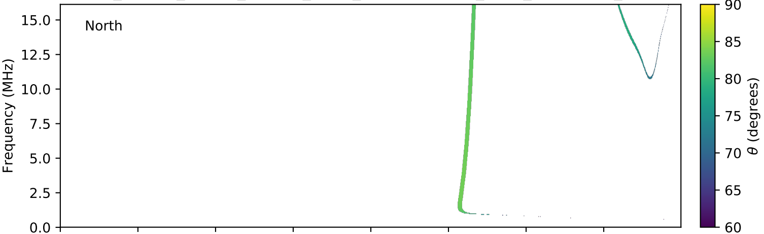
expres_cassini_jupiter_europa_isaac_lossc-wid1deg_3kev_20000405_v01.cdf
