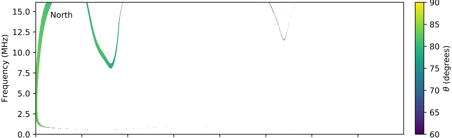
expres_cassini_jupiter_europa_isaac_lossc-wid1deg_3kev_20000402_v01.cdf
