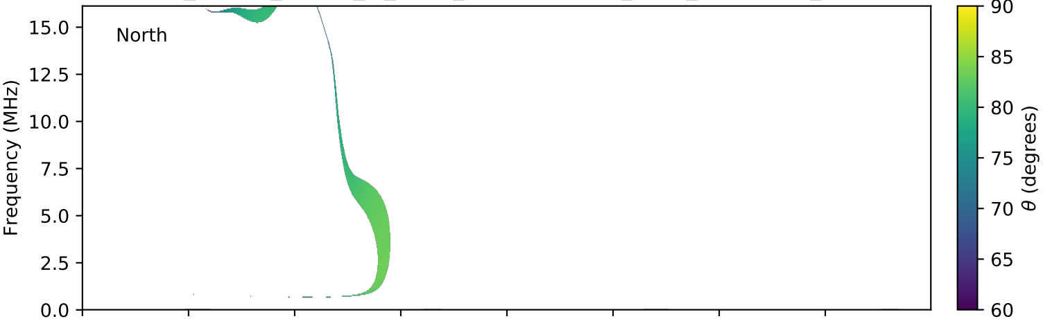
expres_cassini_jupiter_io_isaac_lossc-wid1deg_3kev_20000331_v01.cdf
