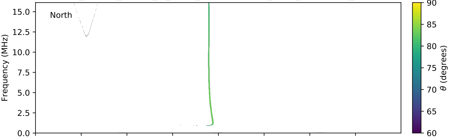
expres_cassini_jupiter_io_isaac_lossc-wid1deg_3kev_20000322_v01.cdf
