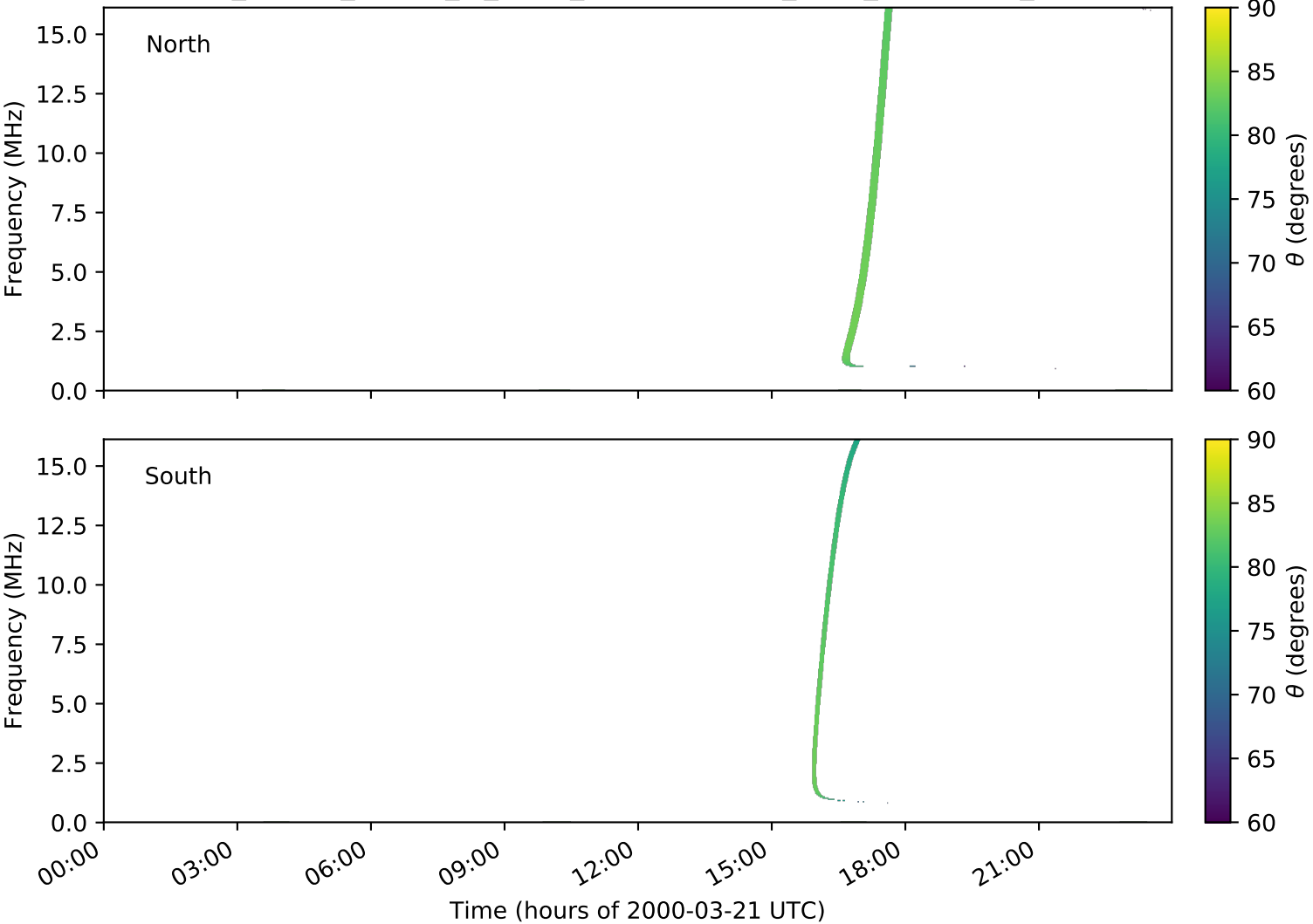
expres_cassini_jupiter_io_isaac_lossc-wid1deg_3kev_20000321_v01.cdf
