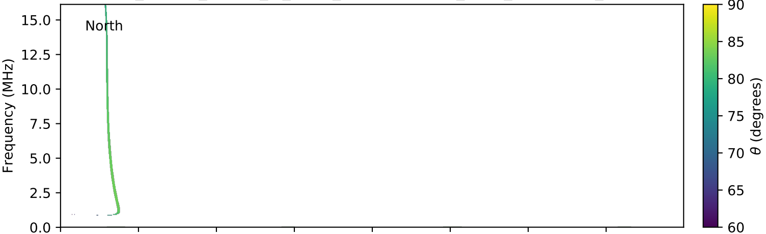
expres_cassini_jupiter_io_isaac_lossc-wid1deg_3kev_20000310_v01.cdf
