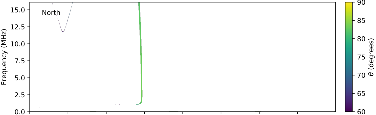
expres_cassini_jupiter_io_isaac_lossc-wid1deg_3kev_20000308_v01.cdf
