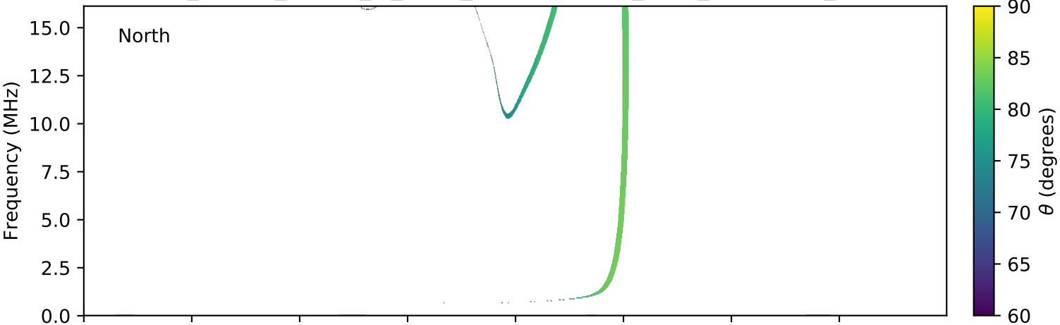
expres_cassini_jupiter_io_isaac_lossc-wid1deg_3kev_20000306_v01.cdf
