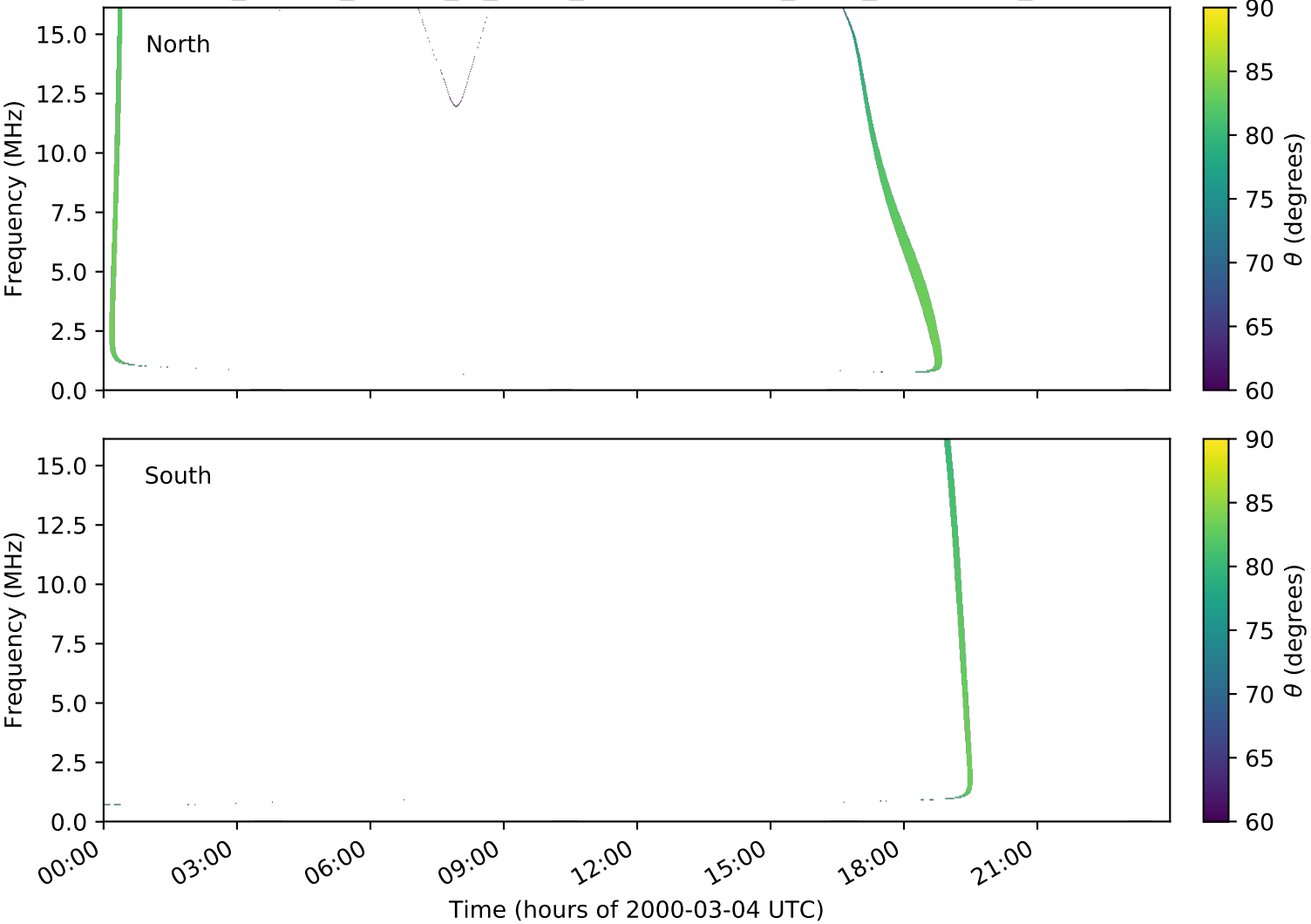
expres_cassini_jupiter_io_isaac_lossc-wid1deg_3kev_20000304_v01.cdf
