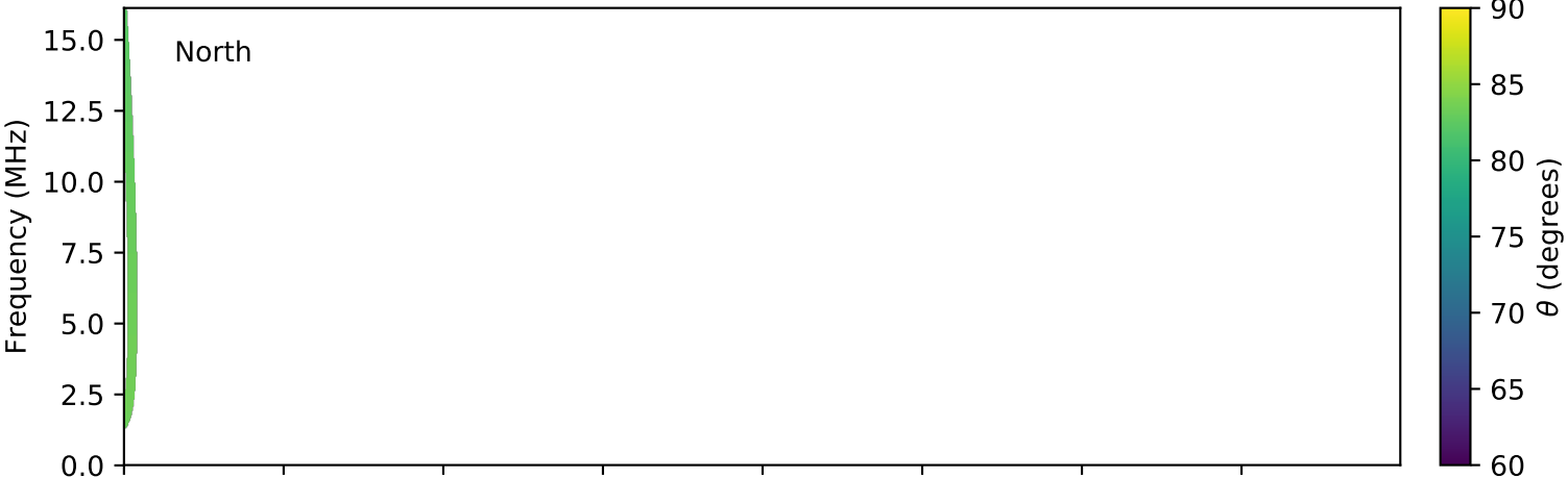
expres_cassini_jupiter_ganymede_isaac_lossc-wid1deg_3kev_20000329_v01.cdf
