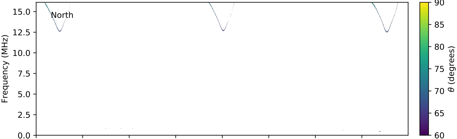
expres_cassini_jupiter_ganymede_isaac_lossc-wid1deg_3kev_20000327_v01.cdf
