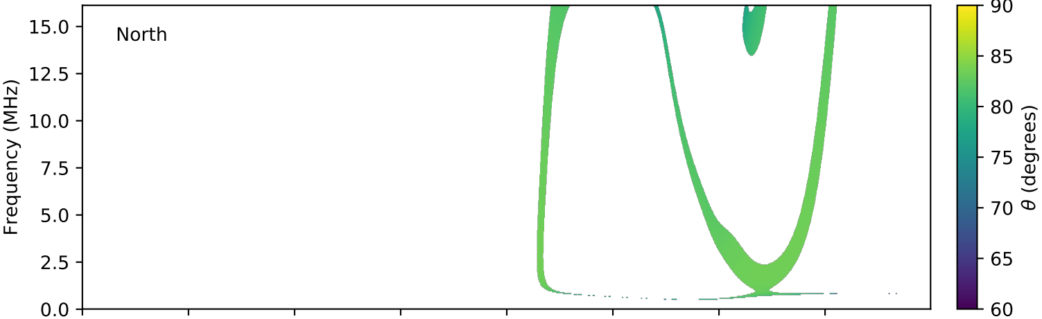
expres_cassini_jupiter_ganymede_isaac_lossc-wid1deg_3kev_20000325_v01.cdf
