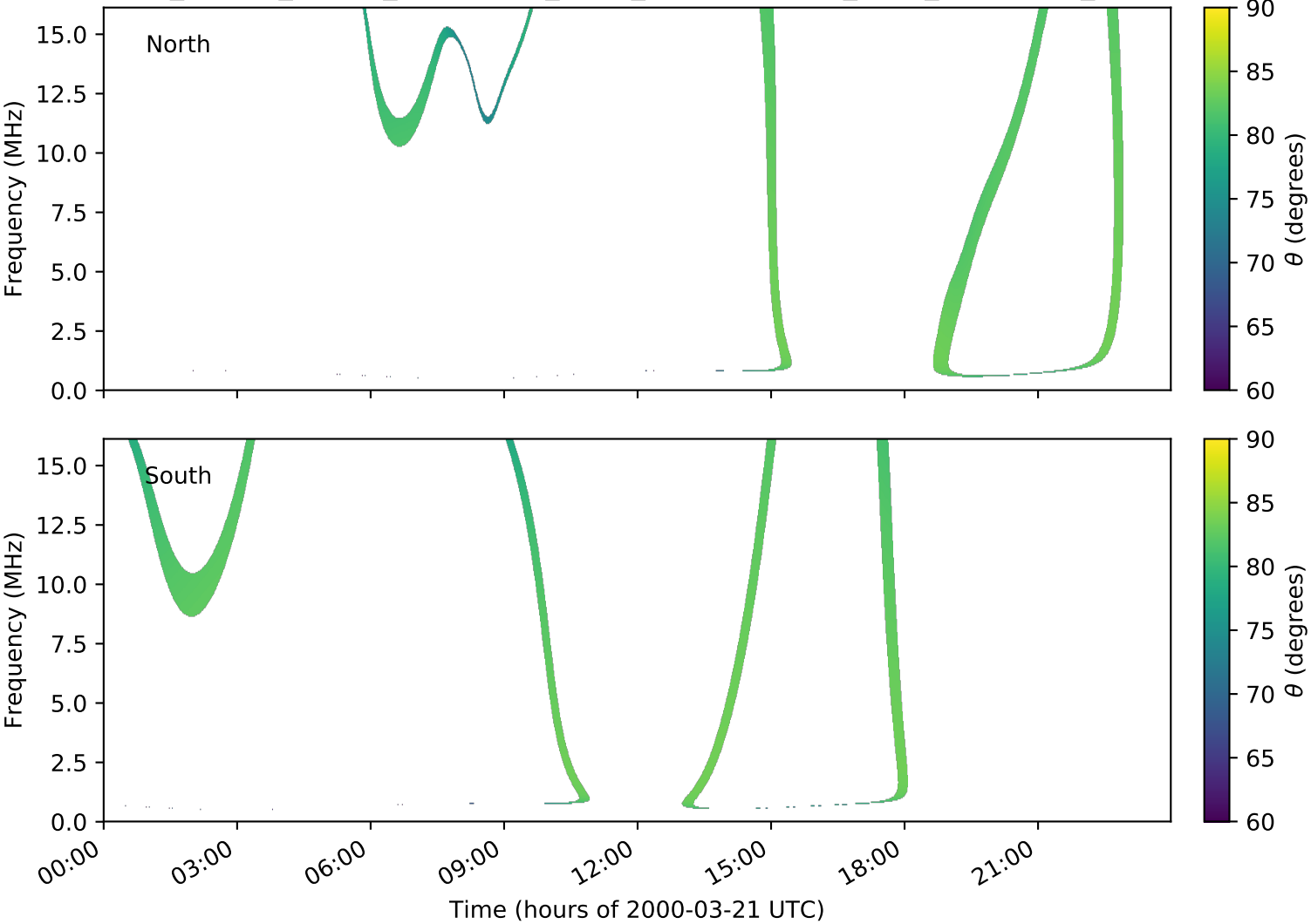
expres_cassini_jupiter_ganymede_isaac_lossc-wid1deg_3kev_20000321_v01.cdf
