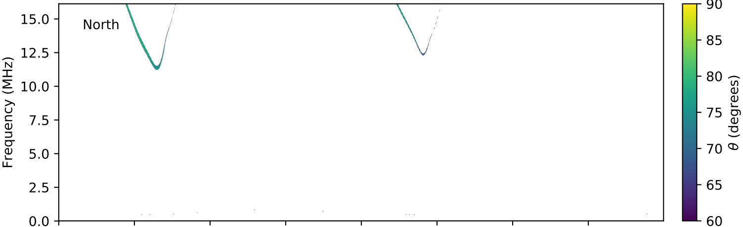
expres_cassini_jupiter_ganymede_isaac_lossc-wid1deg_3kev_20000319_v01.cdf
