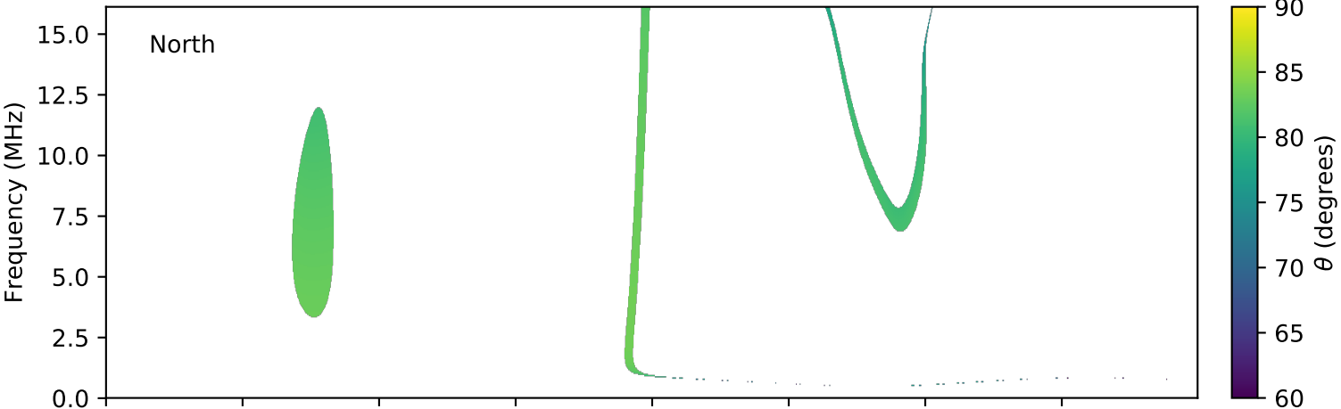
expres_cassini_jupiter_ganymede_isaac_lossc-wid1deg_3kev_20000318_v01.cdf
