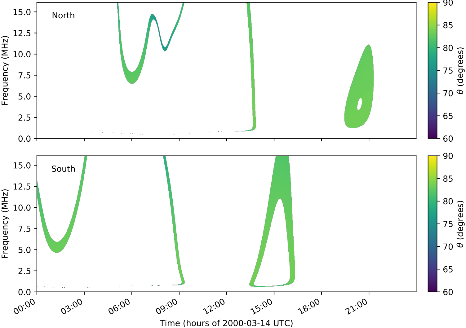
expres_cassini_jupiter_ganymede_isaac_lossc-wid1deg_3kev_20000314_v01.cdf
